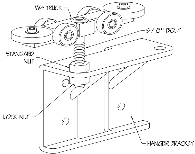
1 GATE HANGER ASSEMBLY HDC-2 Scale: None
