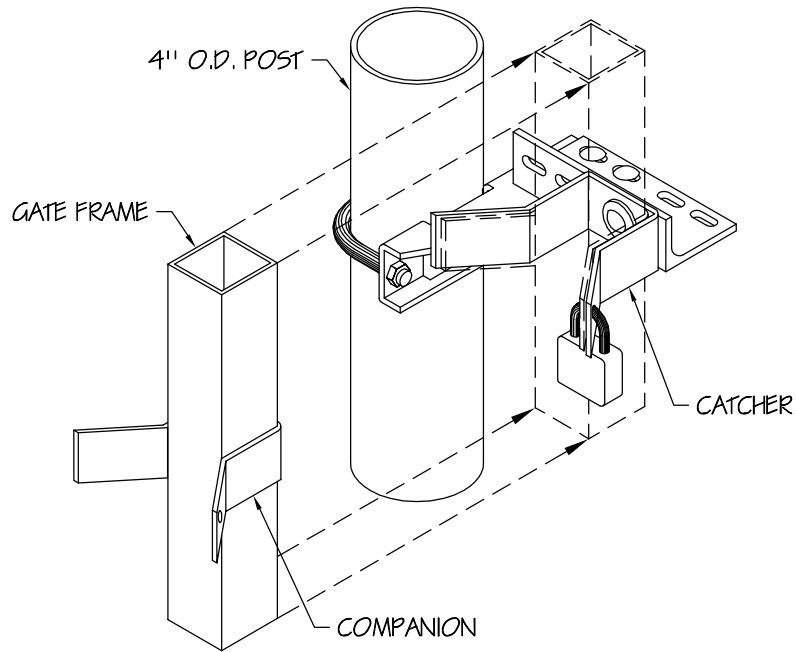
3 CATCH ASSEMBLY HDC-2 Scale: None
